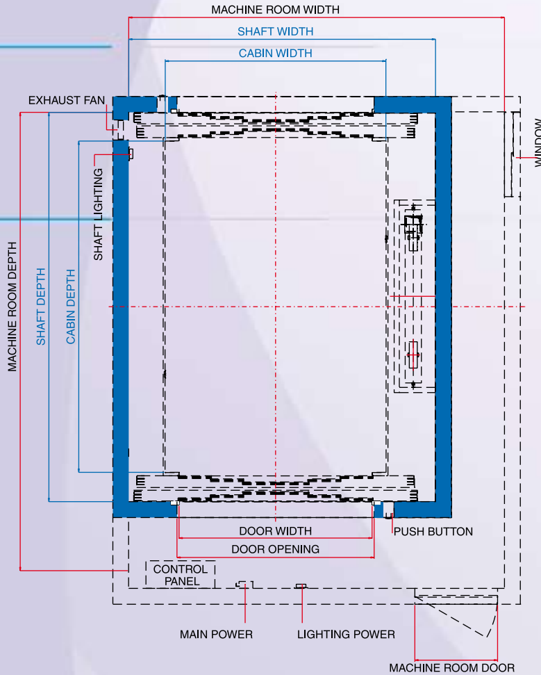
LIFT WELL & MACHINE ROOM
