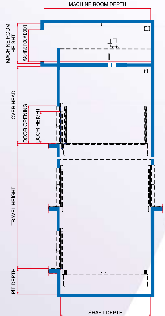
LIFT WELL ELEVATION
